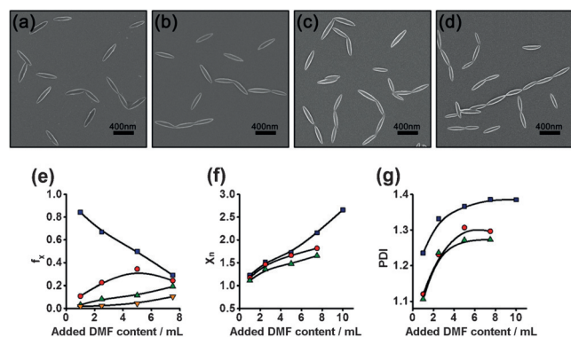
Figure 4. SEM images of nanowire aggregates self-assembled from PBLG-g-PEG subunits with various amounts of DMF added to 10 mL of initial subunit solution (scale bar, 400 nm): a) 1.0 ( \phi_{\text{DMF}} = 0.44 ), b) 2.5 ( \phi_{\text{DMF}} = 0.50 ), c) 5.0 ( \phi_{\text{DMF}} = 0.57 ), and d) 7.5 mL ( \phi_{\text{DMF}} = 0.62 ). e) Number fraction ( f_n ) of the nanowires with various degrees of polymerization (PBLG-g-PEG). Key: X = 1 (—■—), X = 2 (—●—), X = 3 (—▲—), X = 4 (—▼—). f) Number-average degree of polymerization ( X_n ) of the nanowires and g) polydispersity index (PDI) as functions of the amount of DMF added to the initial subunit solution. Degrees of grafting of PBLG-g-PEG, PBLG-g-PEG-1, and PBLG-g-PEG-2 were 1.23%, 2.78%, and 5.90%, respectively. Key (f) and (g): PBLG-g-PEG (—■—), PBLG-g-PEG-1 (—●—), PBLG-g-PEG-2 (—▲—).
