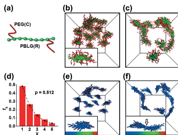
Figure 2. a) DPD model of a rod-g-coil graft copolymer. b,c) Simulation snapshots of spindle-like subunits ( a_{RS}=45 and a_{CS}=25 ) and nanowire aggregates ( a_{RS}=100 and a_{CS}=20 ), where a_{RC}=40 . d) Number fraction ( f_x ) of the nanowires with degree of polymerization ( X ) as a function of X . The dashed line is the theoretical values of f_x . e) Distribution of conservative energy in the subunits under new solvent conditions ( a_{RS}=100 and a_{CS}=20 ), where the insert shows the energy distribution of a single subunit. The colors range from blue (low-energy region) to red (high-energy region). f) Distribution of conservative energy in nanowire aggregates at final equilibrium. The arrow in the insert indicates that the high energy disappears at the connection part of two spindle-like micelles.
